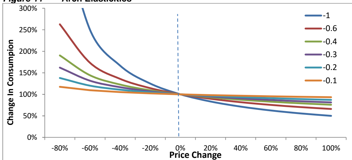
Figure 11 Arch Elasticities
