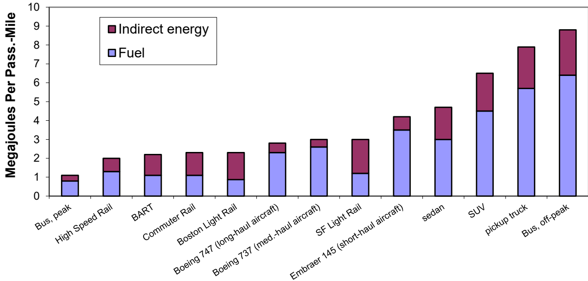
Fuel and embodied energy (energy used in vehicle and facility construction) for various modes.
